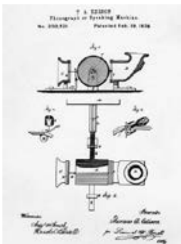
Fig. 2.2. Patent document for the Phonograph (2)
