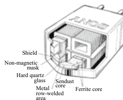
Fig. 9.8. S&F Head structure (9)
