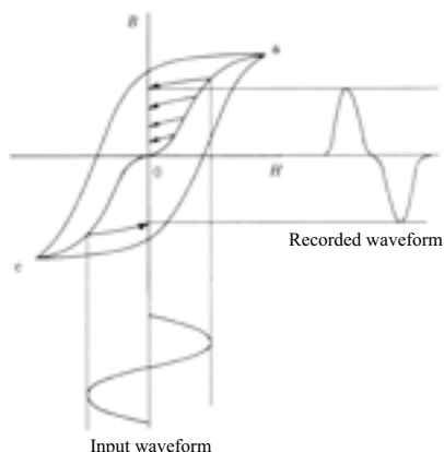
Fig. 3.5. Distortion due to unbiased recording (4)
