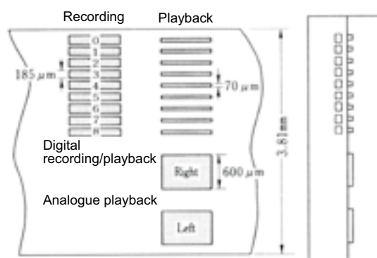
Fig. 14.13. DCC track pattern (13)
