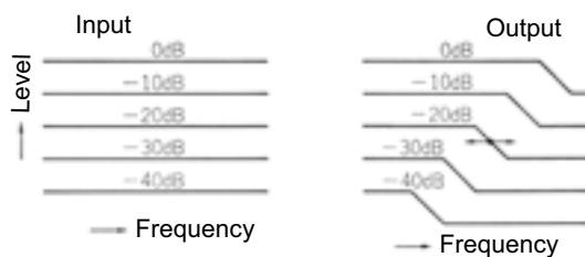
Fig. 11.3. Decoding using the sliding-band method (3)
