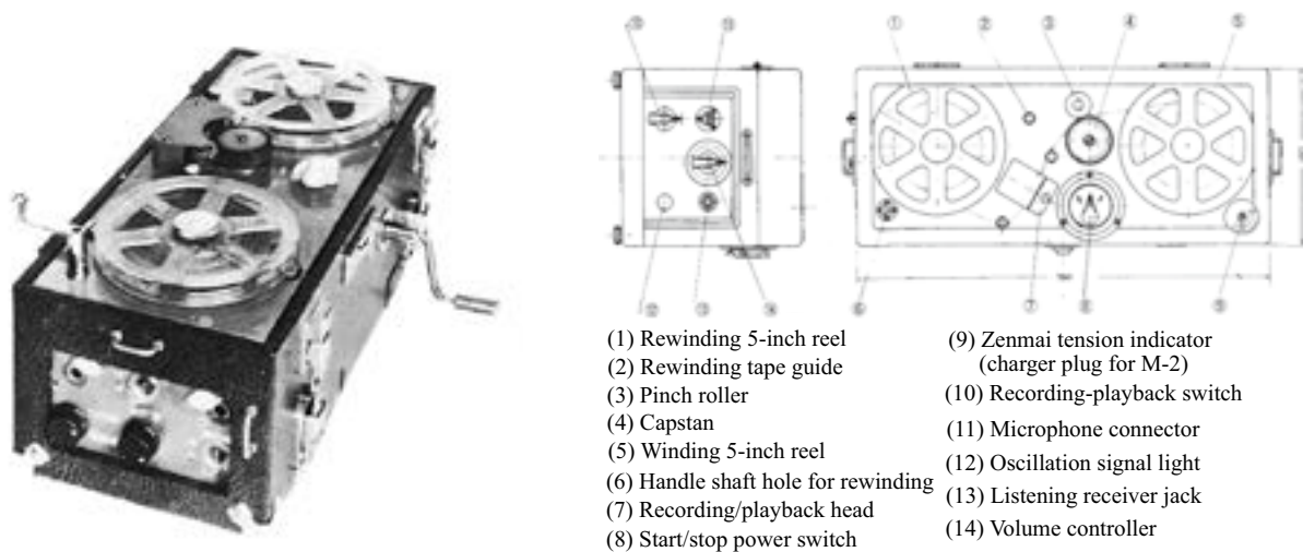
Fig. 5.11. Photograph and exterior diagram of Totsuko M-1 (1951) (12)
