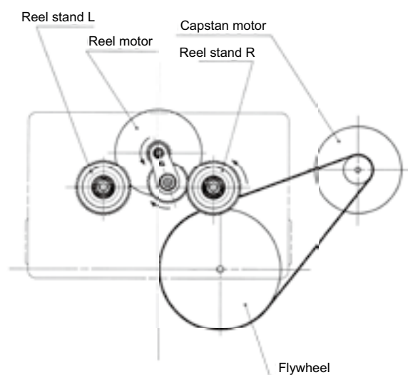
Fig. 12.8. Basic two-motor tape deck mechanism (8)
