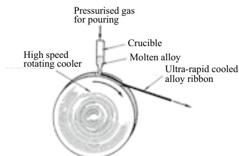
Fig. 9.12. Diagram of the rapid cooling principle (13)
