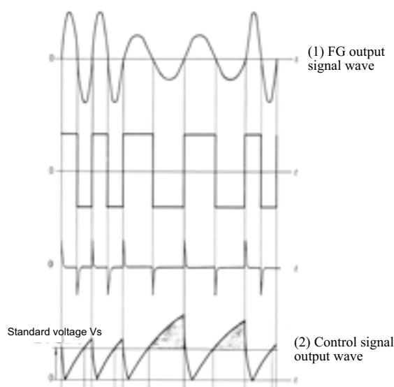
Fig. 12.7. FG output signal processing (section) (7)
