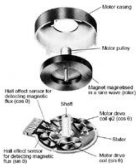
Fig. 12.16. Standard BSL motor
