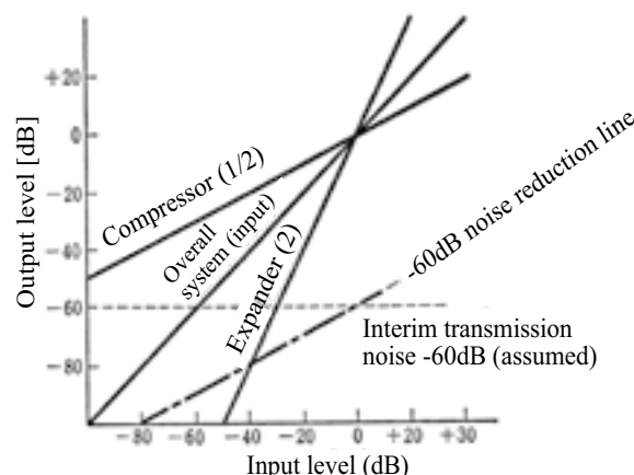
Fig. 11.7. Input and output properties using dbx format (5)
