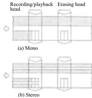
Fig. 6.7. Compact Cassette track arrangement (7)
