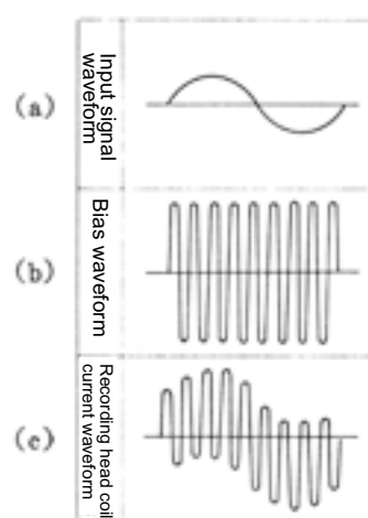
Fig. 3.14. AC bias recording waveforms (14)
