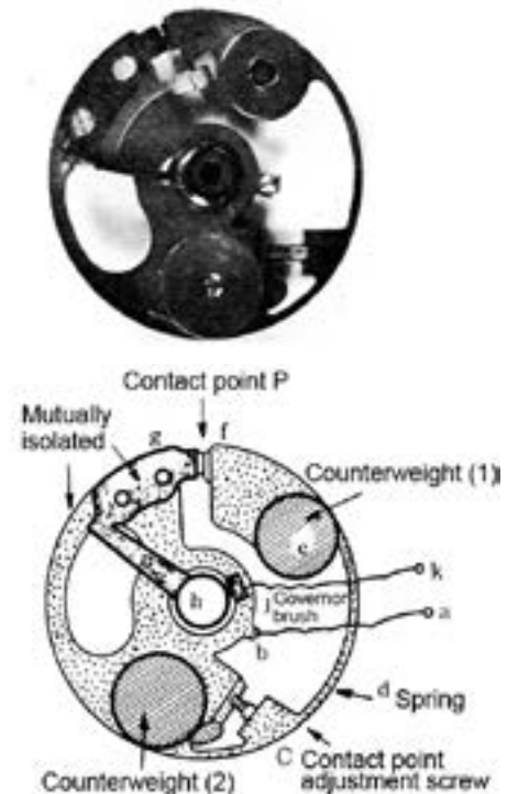
Fig. 12.3. Mechanical Governor (3)
