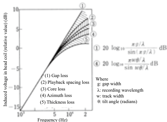
Fig. 7.5. Losses during playback (5)
