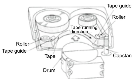
Fig. 14.16. Non-loading mechanism (15)
