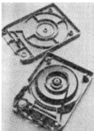
Fig. 6.4. Learjet eight-track cartridge (1965) (4) 102 x 136 x 22mm eight-track/two-channel
