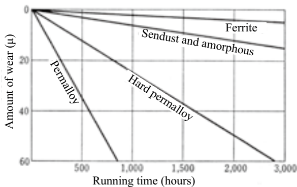
Fig. 9.5. Wear properties according to head material (5)
