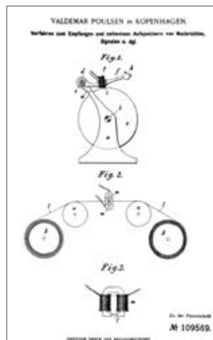
Fig. 3.3. Poulsen's Telegraphone patent (2)
